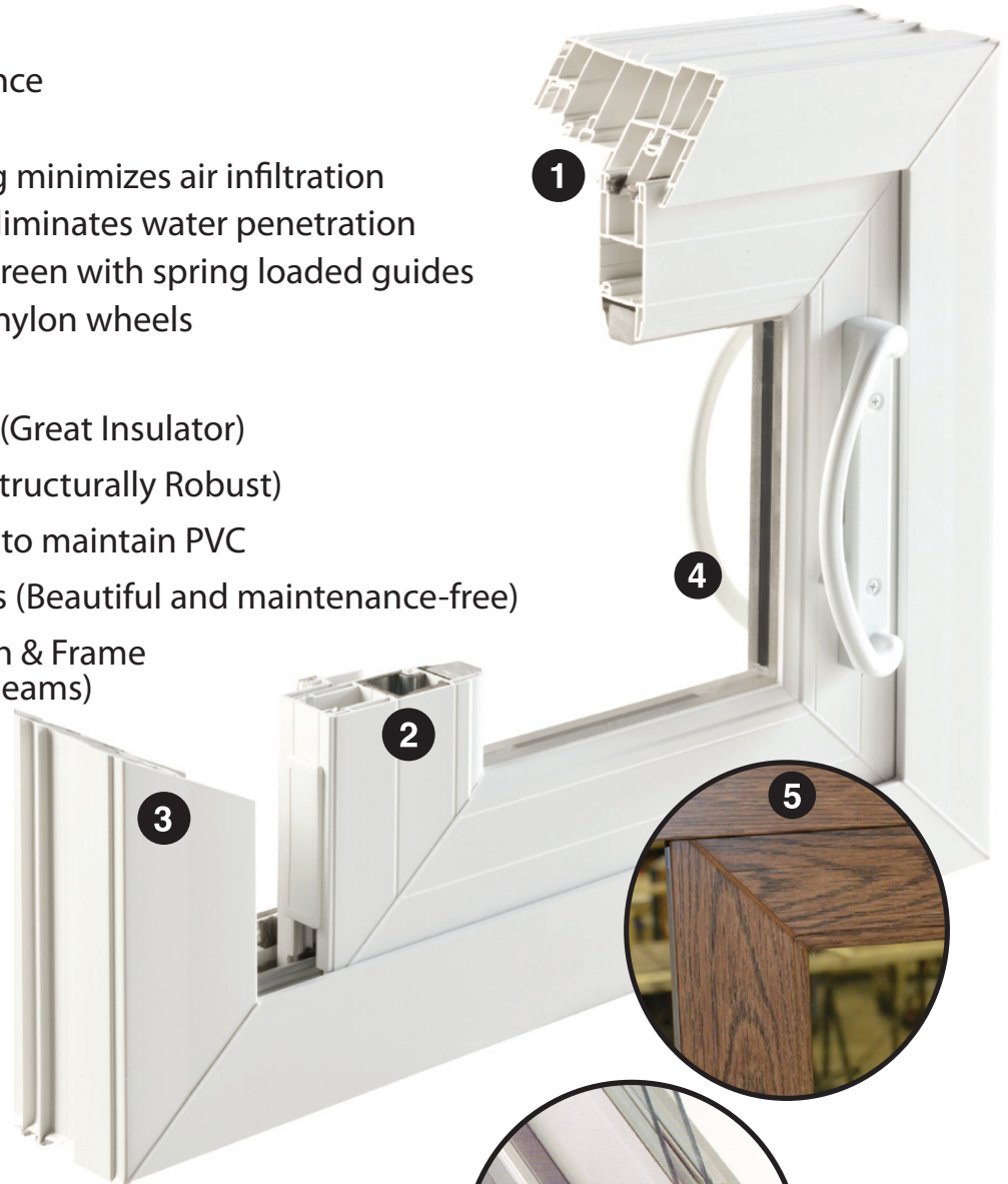
A typical patio door.
